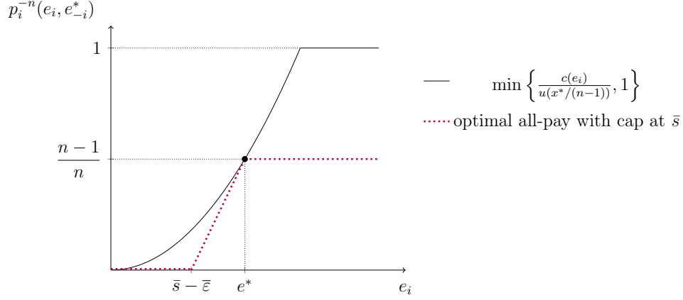
Figure 3: Probability that agent i wins a positive prize when deviating from e^* in the optimal all-pay contest with a cap for i.i.d. additive noise \varepsilon_i \sim U[-0.1, 0.1] , calculated for n = 2 and u(t) = \sqrt{t} and c(e) = e^2 .
